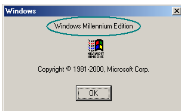
Figure 6 : Windows Millennium
